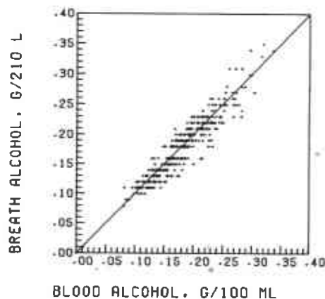
FIG. 3—Scatter plot of Intoxilyzer 5000 results adjusted to a 2300:1 blood/breath alcohol ratio versus blood-alcohol results. The line of 1:1 correlation is shown for reference.
